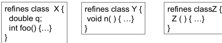
Fig. 9. Crosscutting Example in FOP
