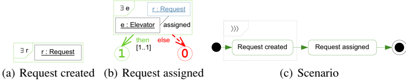
Fig. 11. Deriving a TSSD
