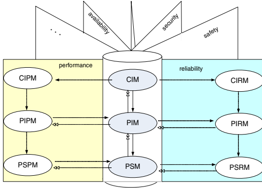
Fig. 2. Views of the NFMDA framework
