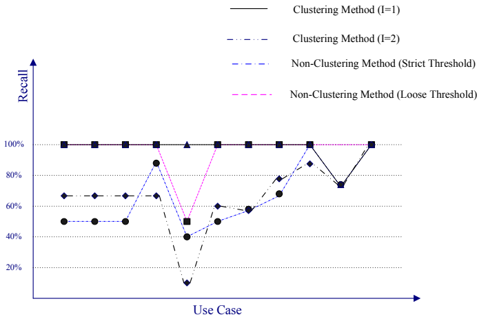
Fig. 2. Comparing clustering-based approach and non-clustering approach
