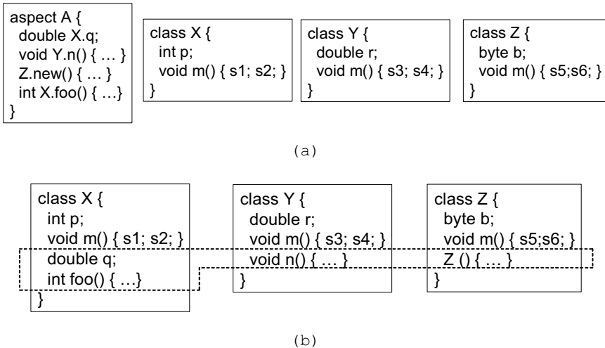
Fig. 1. Static Crosscut Example
