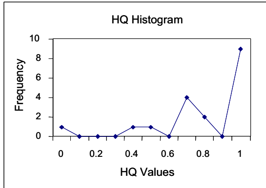
Fig. 7. Prevayler Homogeneity Quotient Histogram
