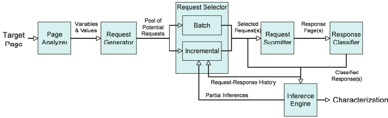
Fig. 1. WebAppSleuth architecture
