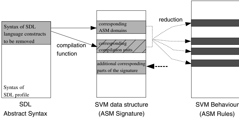
Fig. 1. Concept of the extraction process
