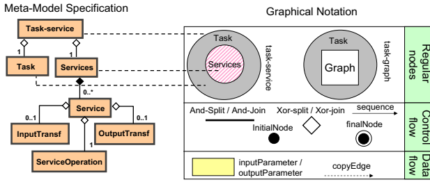
Fig. 1. The composition language
