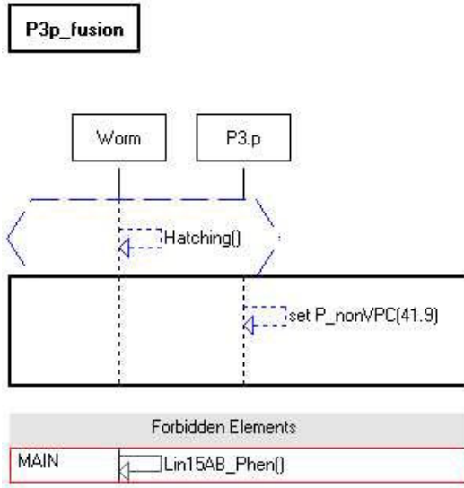
Fig. 4. Activated LSC
