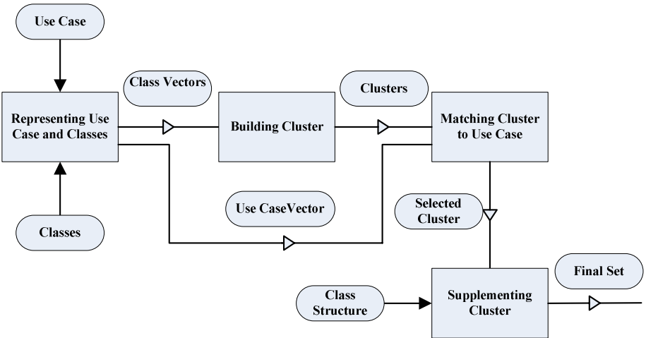
Fig. 1. Approach Overview
